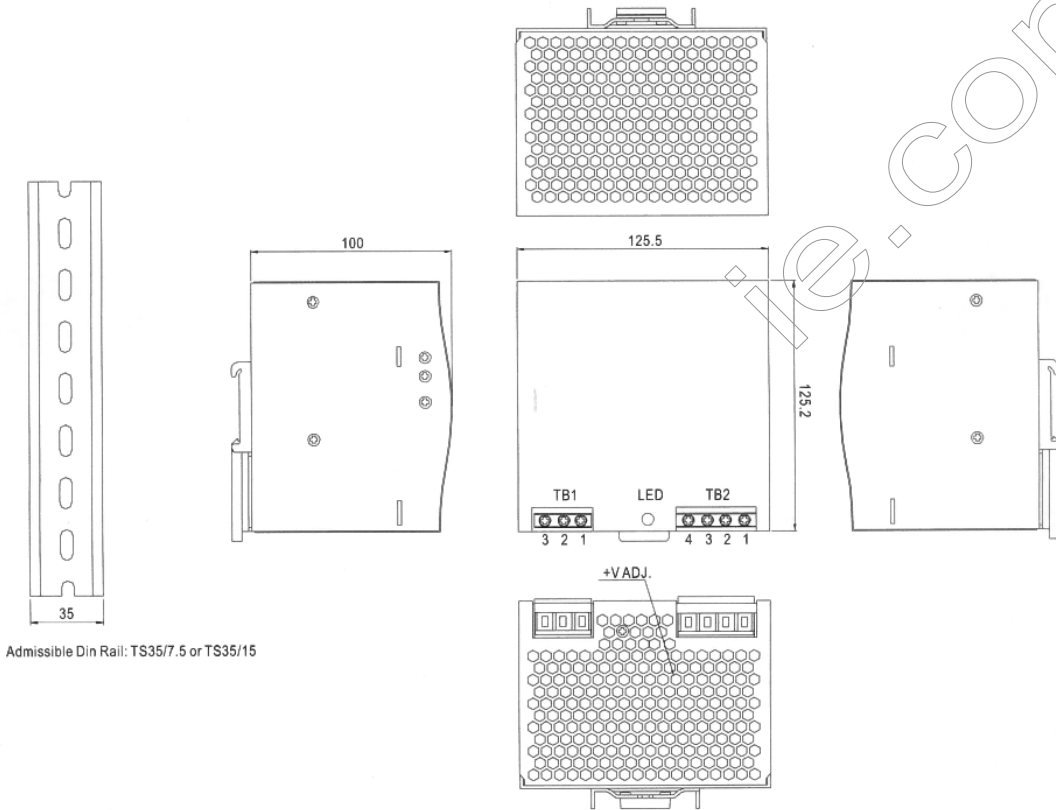
Terminal Pin. No Assignment (TB1)
